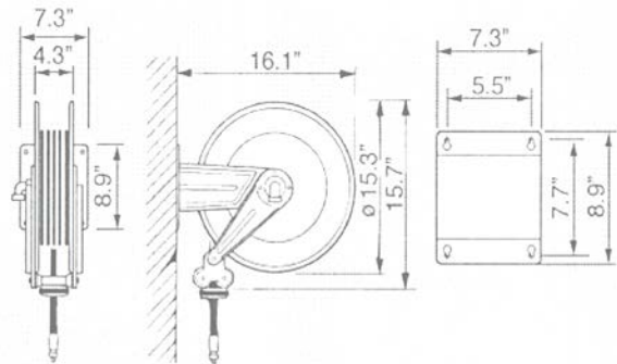
Overall dimensions
